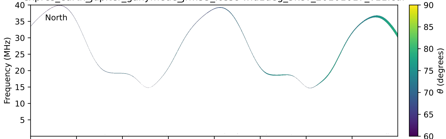
expres_earth_jupiter_ganymede_jrm33_lossc-wid1deg_3kev_20101017_v11.cdf
