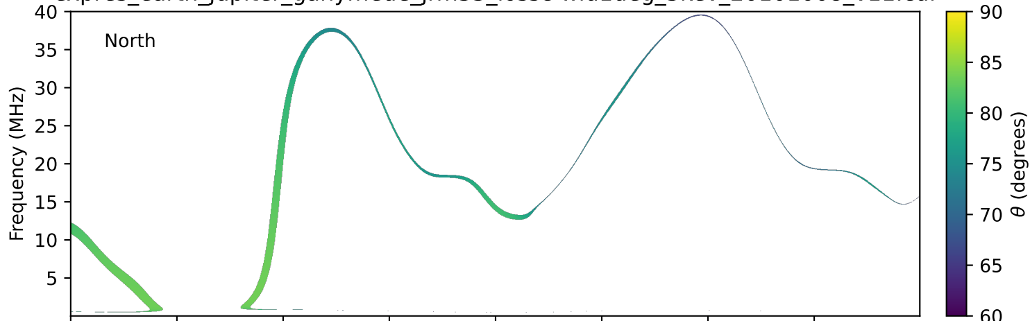
expres_earth_jupiter_ganymede_jrm33_lossc-wid1deg_3kev_20101008_v11.cdf
