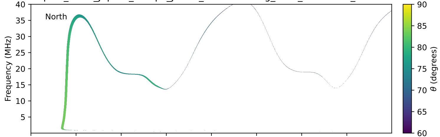
expres_earth_jupiter_europa_jrm33_lossc-wid1deg_3kev_20101009_v11.cdf
