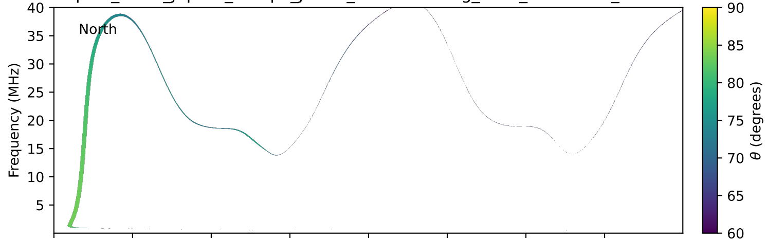
expres_earth_jupiter_europa_jrm33_lossc-wid1deg_3kev_20101002_v11.cdf
