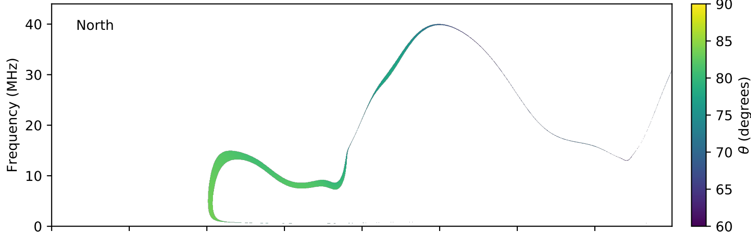
expres_earth_jupiter_europa_jrm09_lossc-wid1deg_3kev_20101030_v01.cdf
