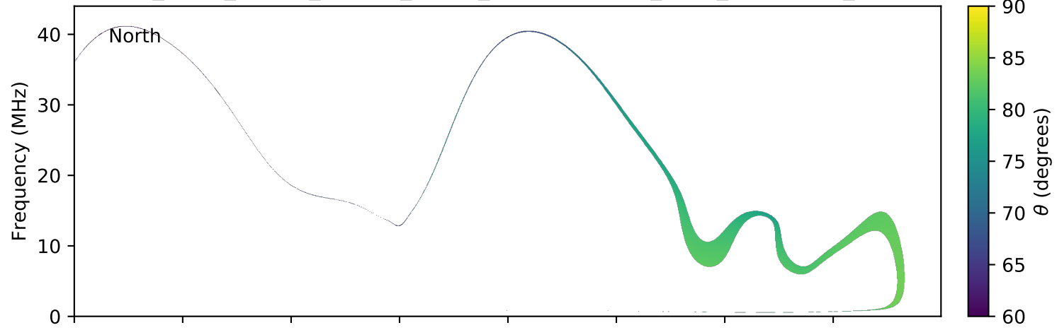
expres_earth_jupiter_europa_jrm09_lossc-wid1deg_3kev_20101024_v01.cdf
