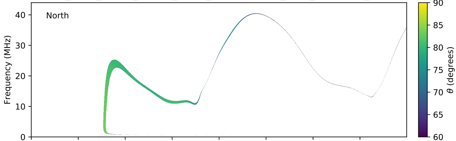
expres_earth_jupiter_europa_jrm09_lossc-wid1deg_3kev_20101023_v01.cdf
