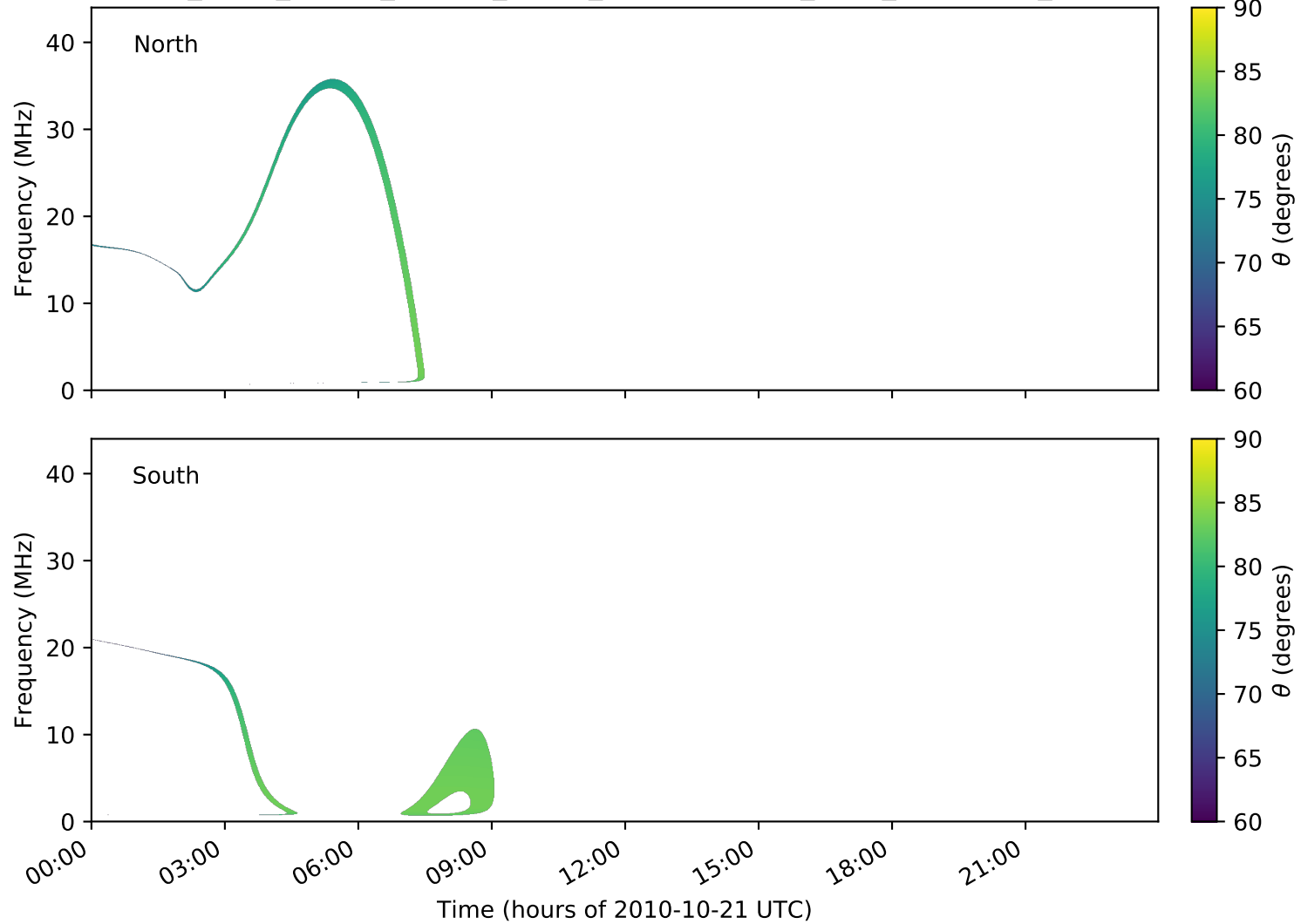
expres_earth_jupiter_europa_jrm09_lossc-wid1deg_3kev_20101021_v01.cdf
