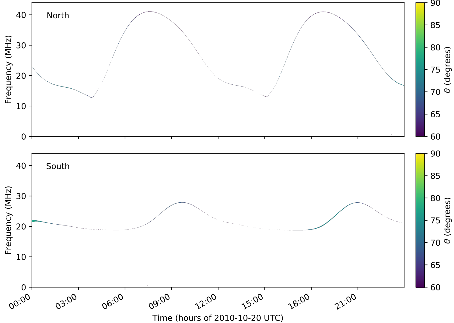
expres_earth_jupiter_europa_jrm09_lossc-wid1deg_3kev_20101020_v01.cdf
