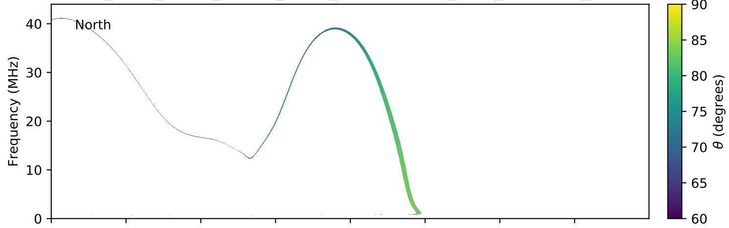
expres_earth_jupiter_europa_jrm09_lossc-wid1deg_3kev_20101010_v01.cdf
