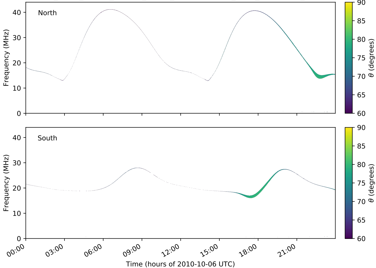
expres_earth_jupiter_europa_jrm09_lossc-wid1deg_3kev_20101006_v01.cdf
