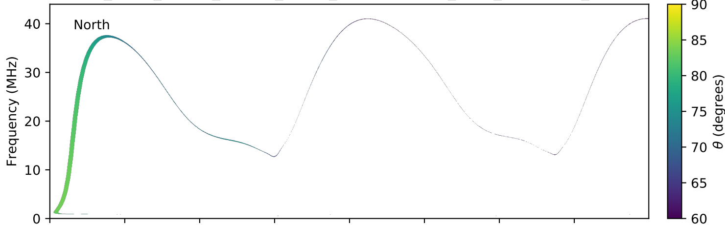
expres_earth_jupiter_europa_jrm09_lossc-wid1deg_3kev_20101002_v01.cdf
