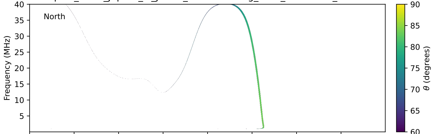
expres_earth_jupiter_io_jrm33_lossc-wid1deg_3kev_20100930_v11.cdf
