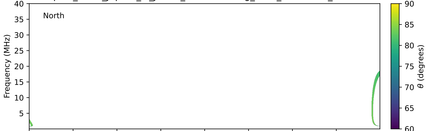
expres_earth_jupiter_io_jrm33_lossc-wid1deg_3kev_20100920_v11.cdf
