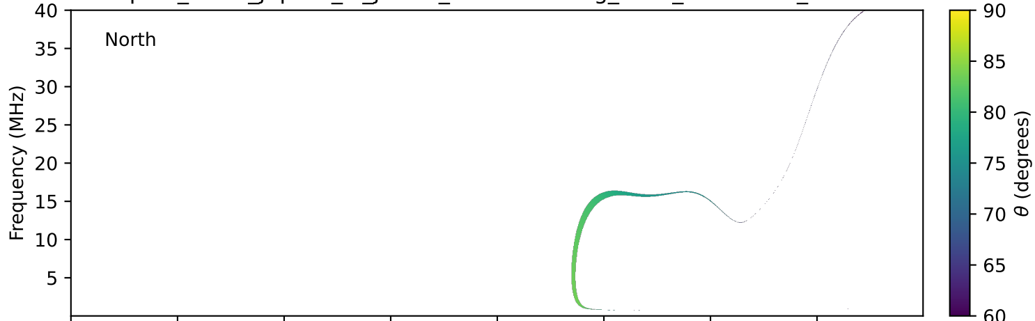
expres_earth_jupiter_io_jrm33_lossc-wid1deg_3kev_20100908_v11.cdf
