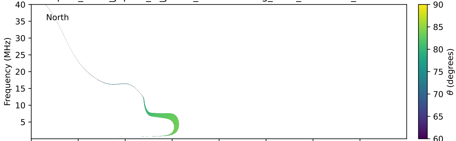
expres_earth_jupiter_io_jrm33_lossc-wid1deg_3kev_20100902_v11.cdf
