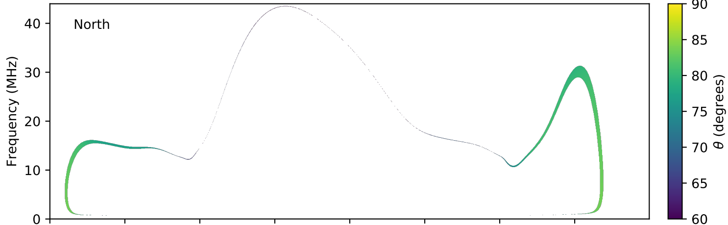
expres_earth_jupiter_io_jrm09_lossc-wid1deg_3kev_20100928_v01.cdf
