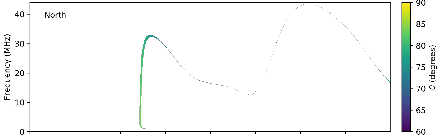
expres_earth_jupiter_io_jrm09_lossc-wid1deg_3kev_20100926_v01.cdf
