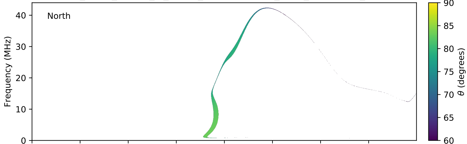
expres_earth_jupiter_io_jrm09_lossc-wid1deg_3kev_20100917_v01.cdf
