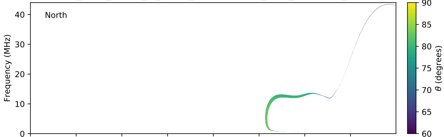
expres_earth_jupiter_io_jrm09_lossc-wid1deg_3kev_20100915_v01.cdf
