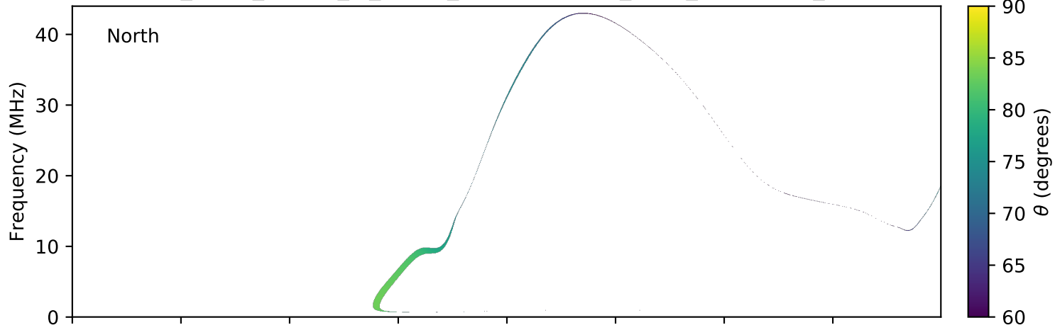
expres_earth_jupiter_io_jrm09_lossc-wid1deg_3kev_20100910_v01.cdf
