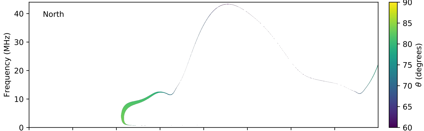
expres_earth_jupiter_io_jrm09_lossc-wid1deg_3kev_20100903_v01.cdf
