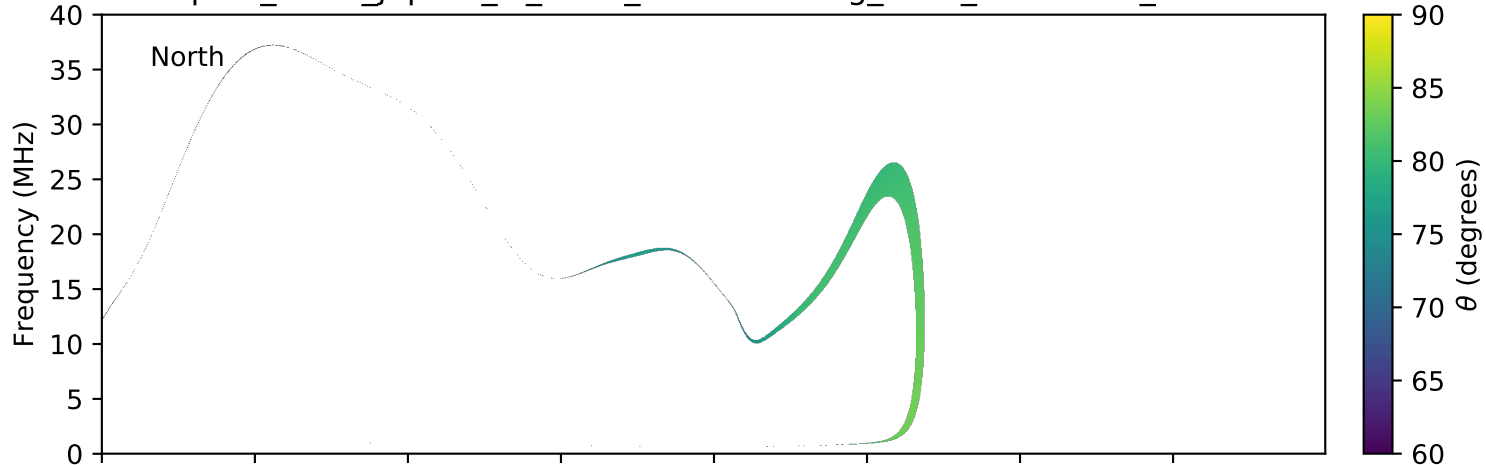
expres_earth_jupiter_io_isaac_lossc-wid1deg_3kev_20100930_v01.cdf
