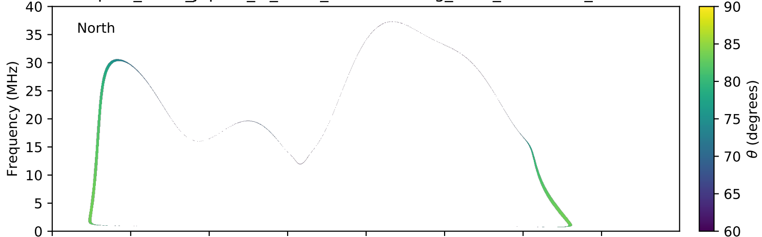
expres_earth_jupiter_io_isaac_lossc-wid1deg_3kev_20100928_v01.cdf
