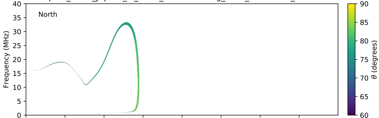
expres_earth_jupiter_io_isaac_lossc-wid1deg_3kev_20100925_v01.cdf
