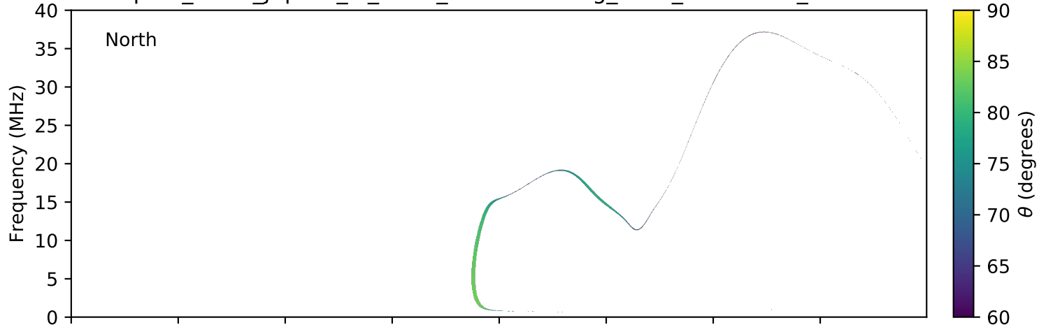
expres_earth_jupiter_io_isaac_lossc-wid1deg_3kev_20100924_v01.cdf
