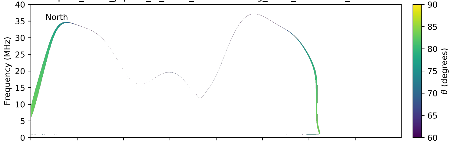
expres_earth_jupiter_io_isaac_lossc-wid1deg_3kev_20100921_v01.cdf
