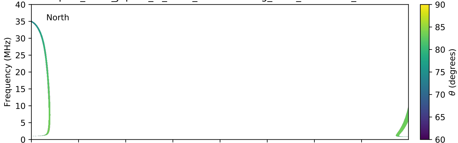
expres_earth_jupiter_io_isaac_lossc-wid1deg_3kev_20100920_v01.cdf
