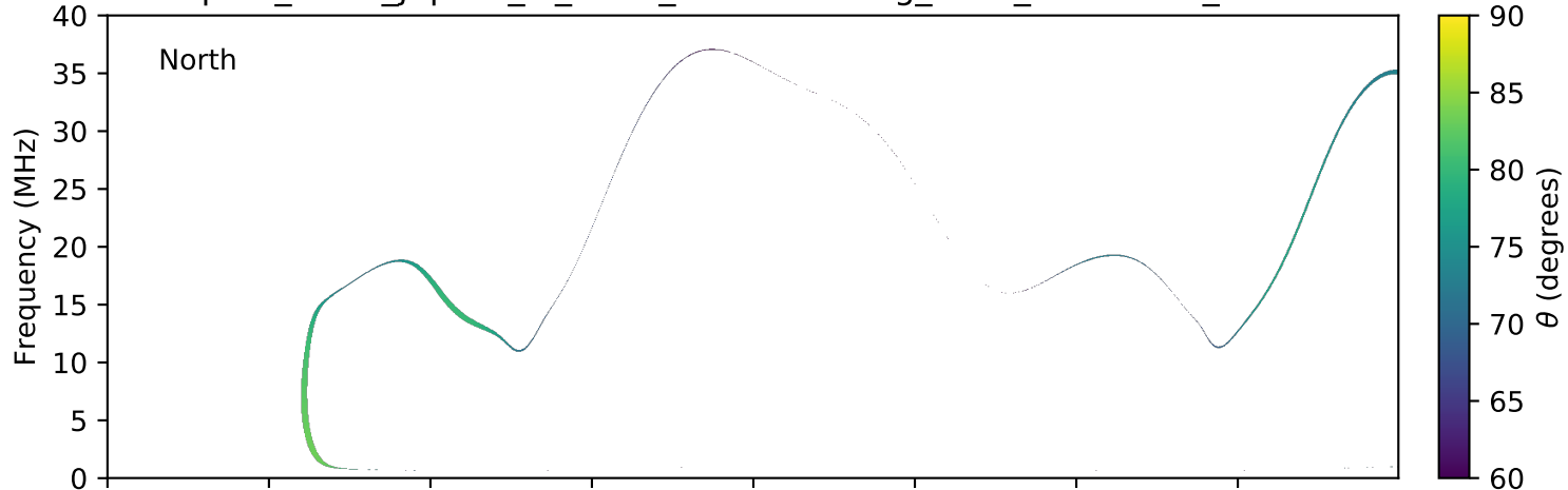
expres_earth_jupiter_io_isaac_lossc-wid1deg_3kev_20100919_v01.cdf
