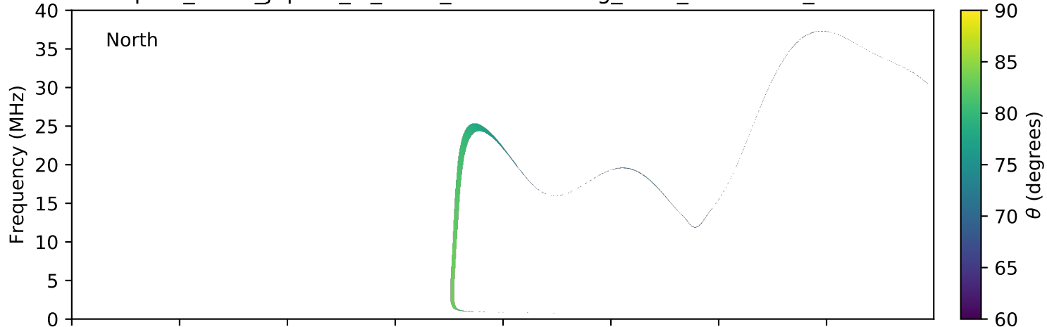
expres_earth_jupiter_io_isaac_lossc-wid1deg_3kev_20100917_v01.cdf
