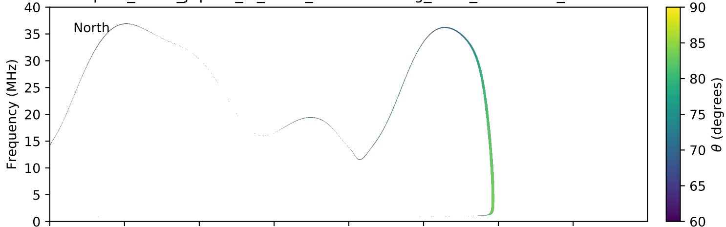
expres_earth_jupiter_io_isaac_lossc-wid1deg_3kev_20100914_v01.cdf
