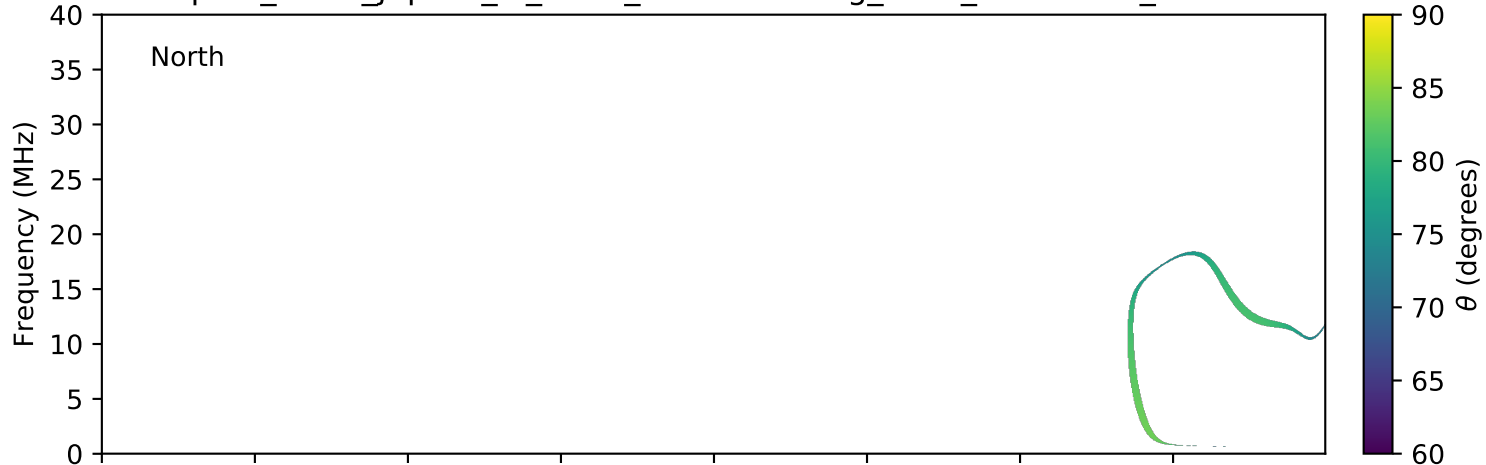
expres_earth_jupiter_io_isaac_lossc-wid1deg_3kev_20100913_v01.cdf
