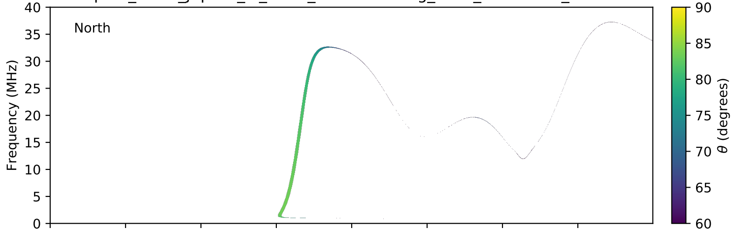
expres_earth_jupiter_io_isaac_lossc-wid1deg_3kev_20100910_v01.cdf
