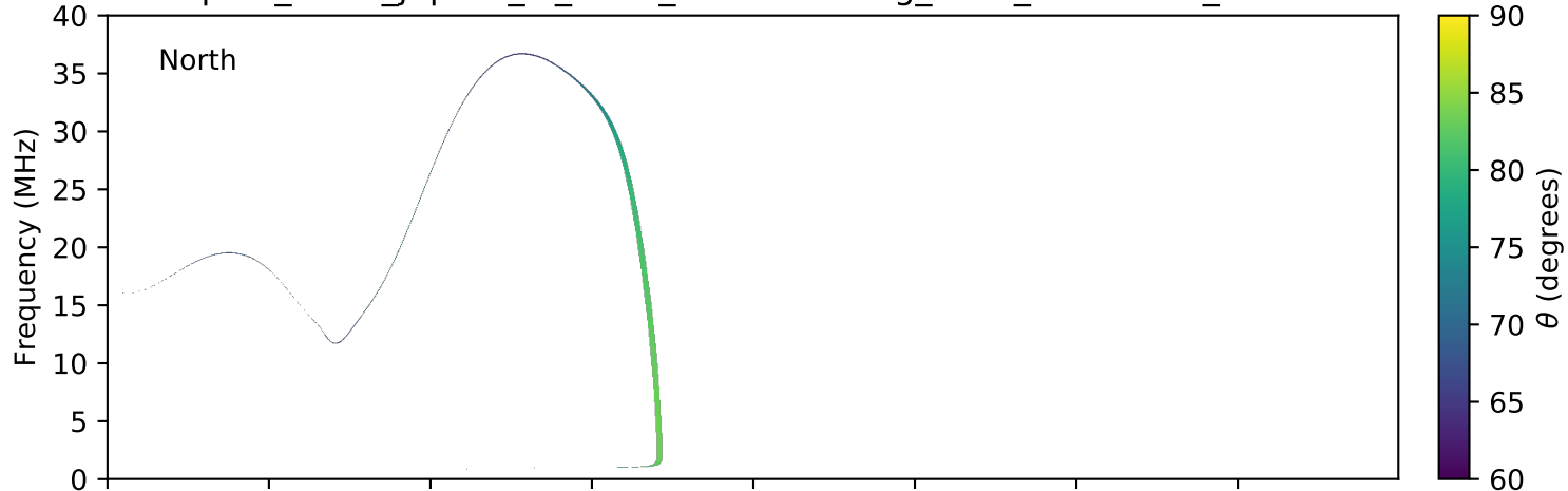
expres_earth_jupiter_io_isaac_lossc-wid1deg_3kev_20100909_v01.cdf
