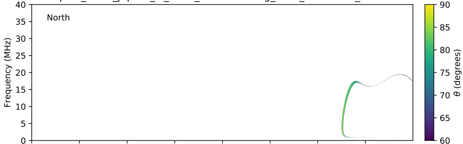
expres_earth_jupiter_io_isaac_lossc-wid1deg_3kev_20100906_v01.cdf
