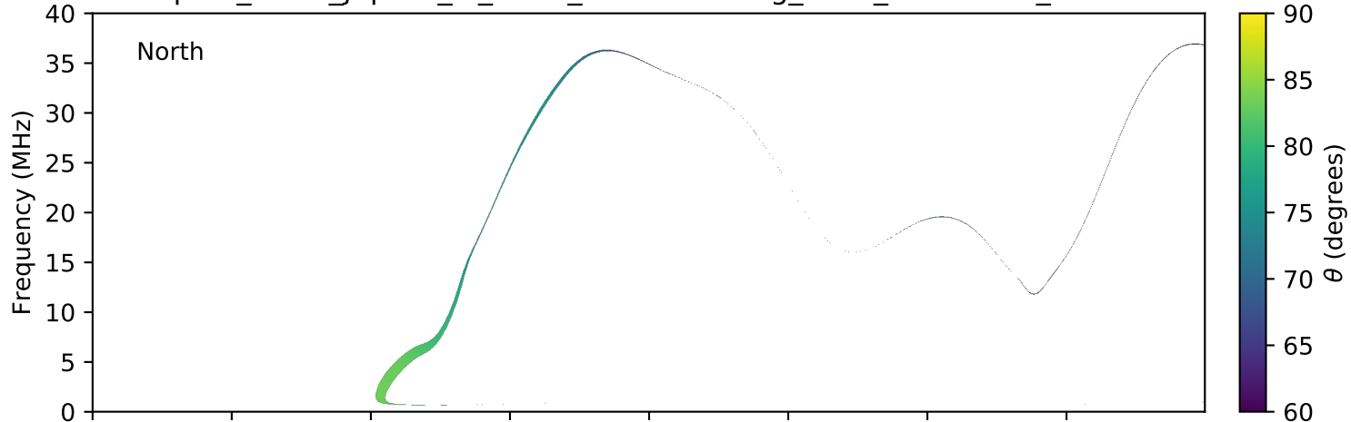
expres_earth_jupiter_io_isaac_lossc-wid1deg_3kev_20100903_v01.cdf
