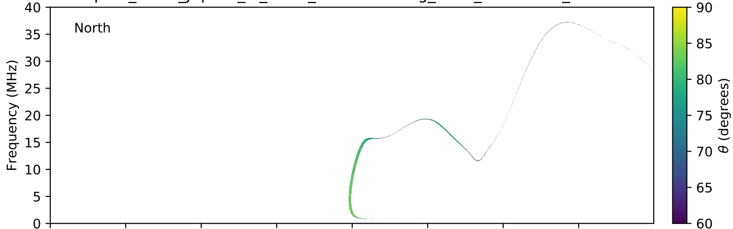
expres_earth_jupiter_io_isaac_lossc-wid1deg_3kev_20100901_v01.cdf
