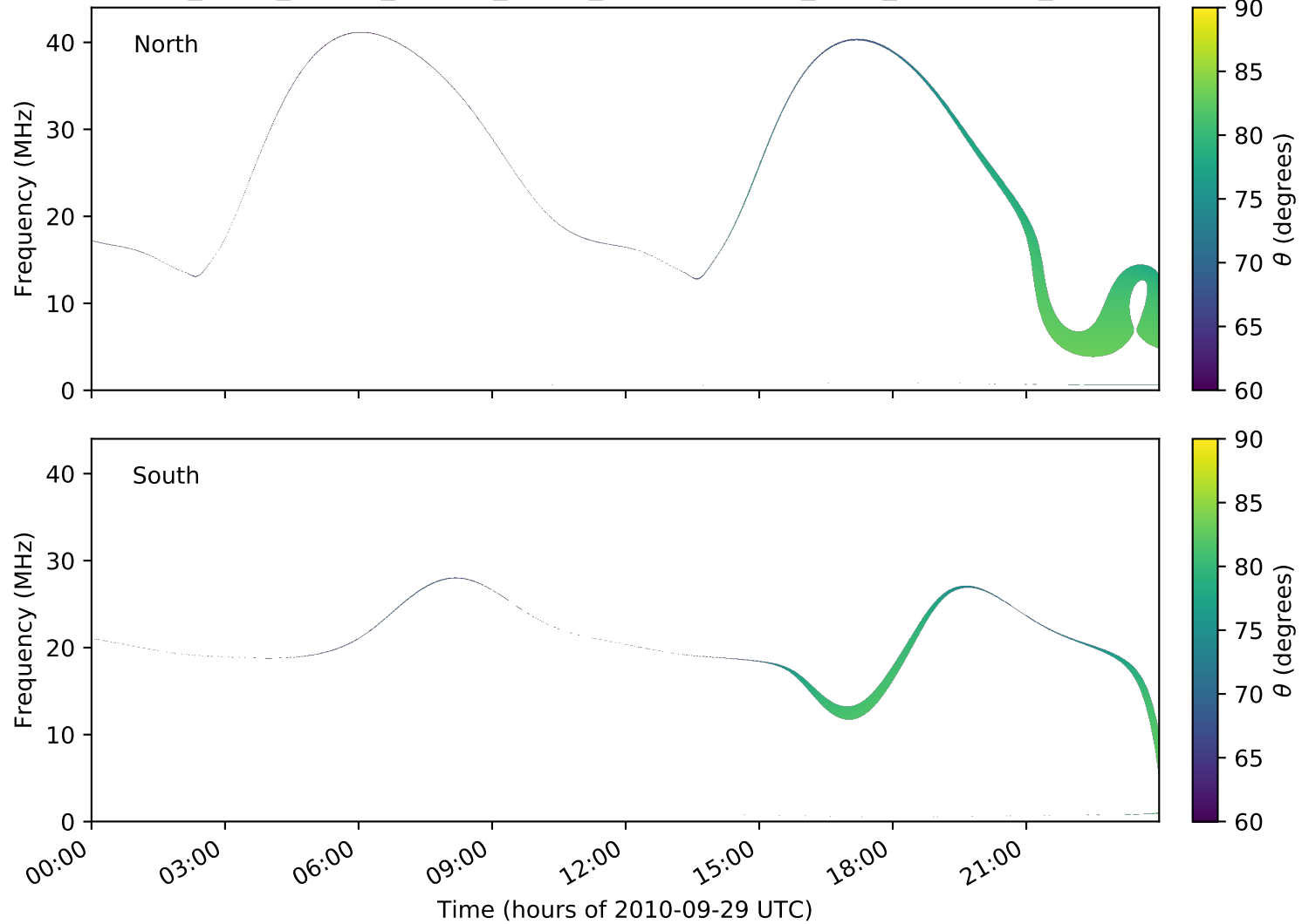
expres_earth_jupiter_europa_jrm09_lossc-wid1deg_3kev_20100929_v01.cdf
