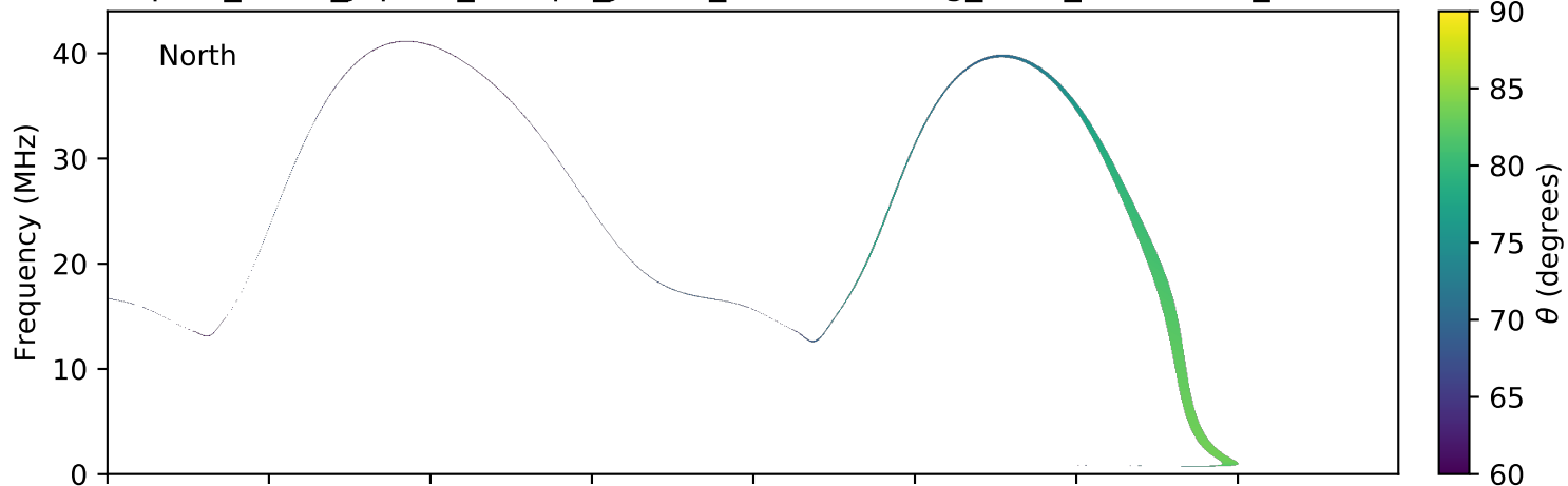
expres_earth_jupiter_europa_jrm09_lossc-wid1deg_3kev_20100922_v01.cdf
