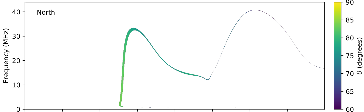
expres_earth_jupiter_europa_jrm09_lossc-wid1deg_3kev_20100921_v01.cdf
