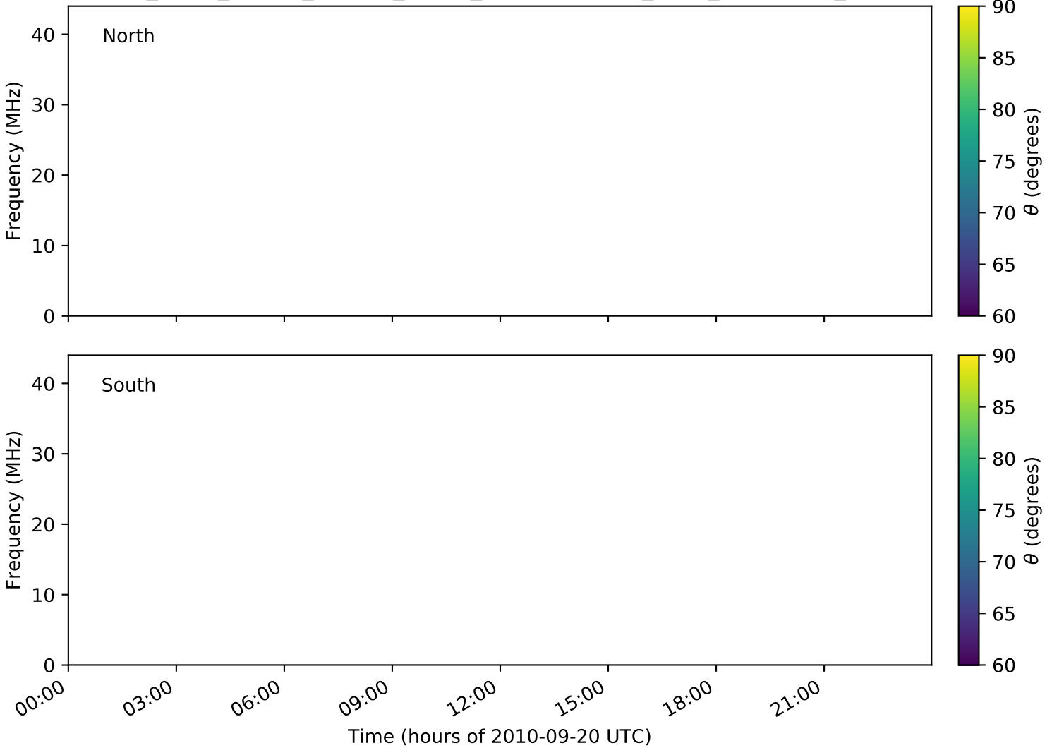
expres_earth_jupiter_europa_jrm09_lossc-wid1deg_3kev_20100920_v01.cdf
