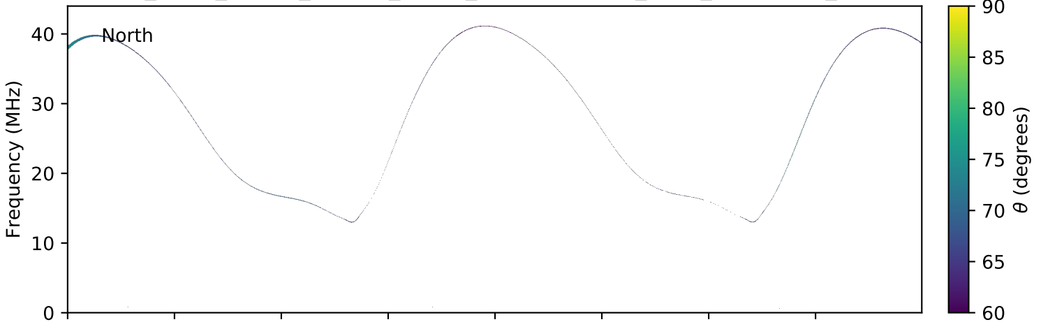
expres_earth_jupiter_europa_jrm09_lossc-wid1deg_3kev_20100918_v01.cdf
