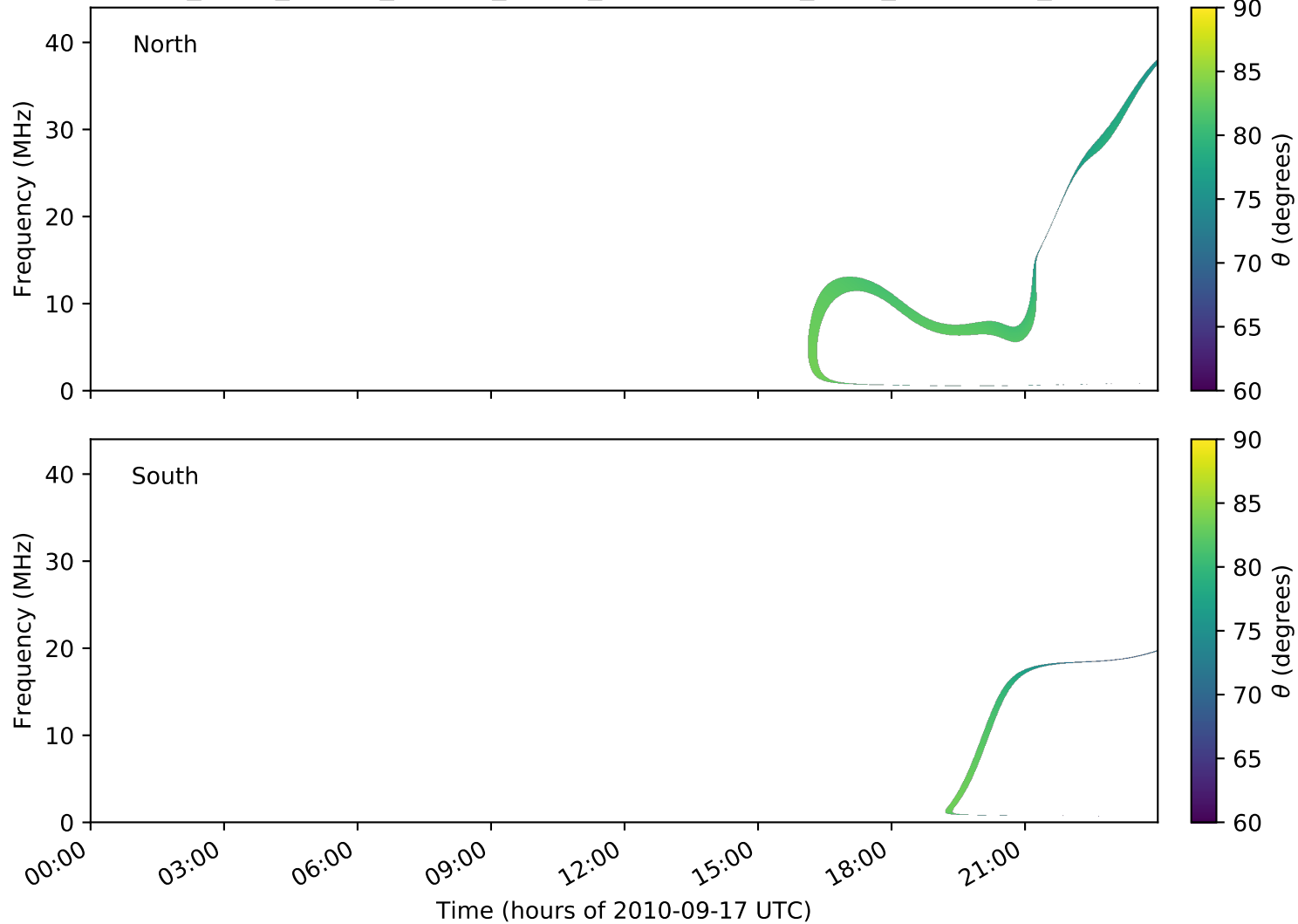
expres_earth_jupiter_europa_jrm09_lossc-wid1deg_3kev_20100917_v01.cdf
