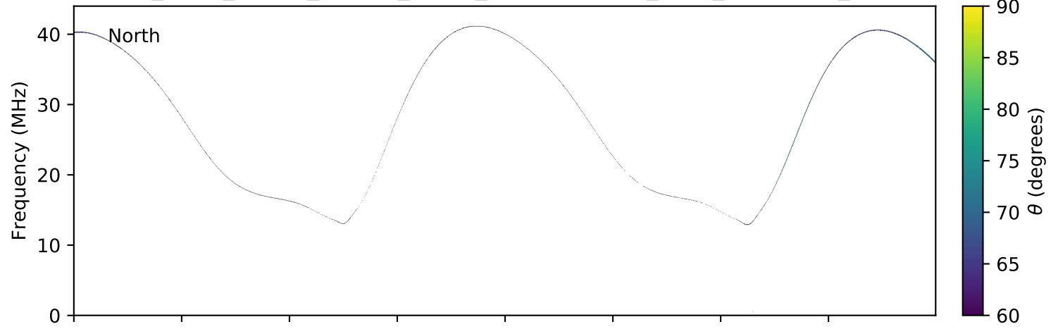
expres_earth_jupiter_europa_jrm09_lossc-wid1deg_3kev_20100911_v01.cdf
