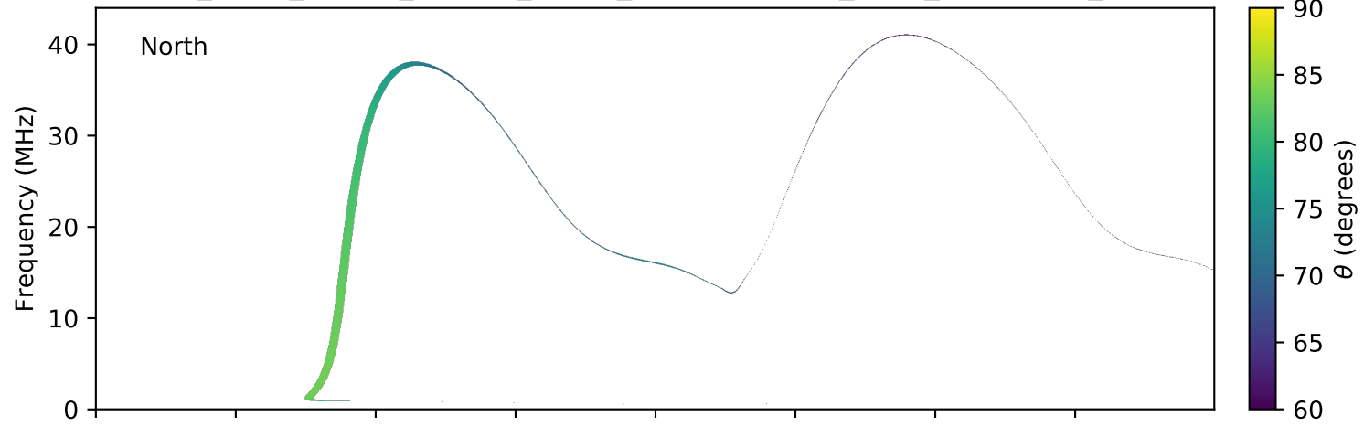
expres_earth_jupiter_europa_jrm09_lossc-wid1deg_3kev_20100907_v01.cdf
