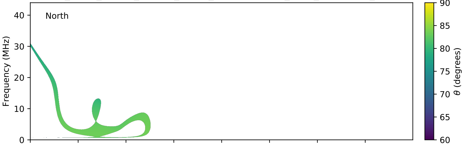
expres_earth_jupiter_europa_jrm09_lossc-wid1deg_3kev_20100905_v01.cdf
