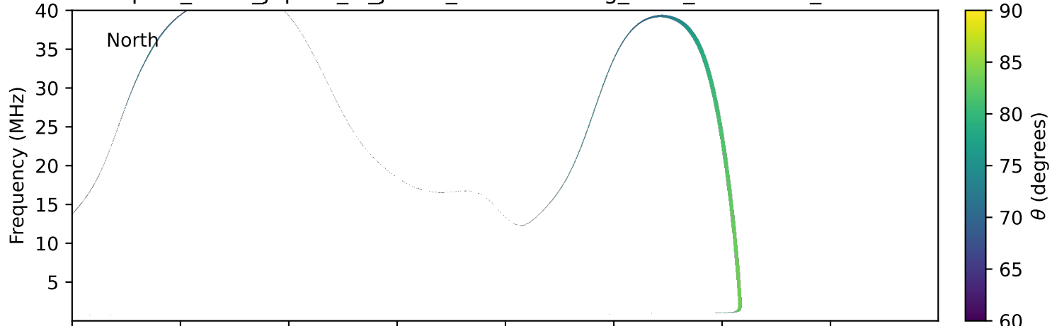
expres_earth_jupiter_io_jrm33_lossc-wid1deg_3kev_20100822_v11.cdf
