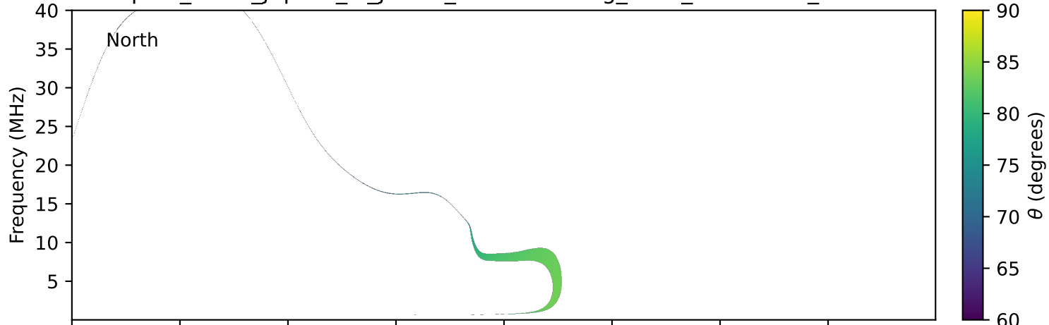
expres_earth_jupiter_io_jrm33_lossc-wid1deg_3kev_20100801_v11.cdf
