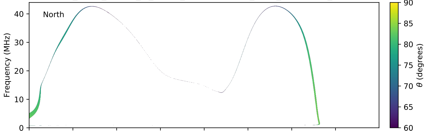
expres_earth_jupiter_io_jrm09_lossc-wid1deg_3kev_20100829_v01.cdf
