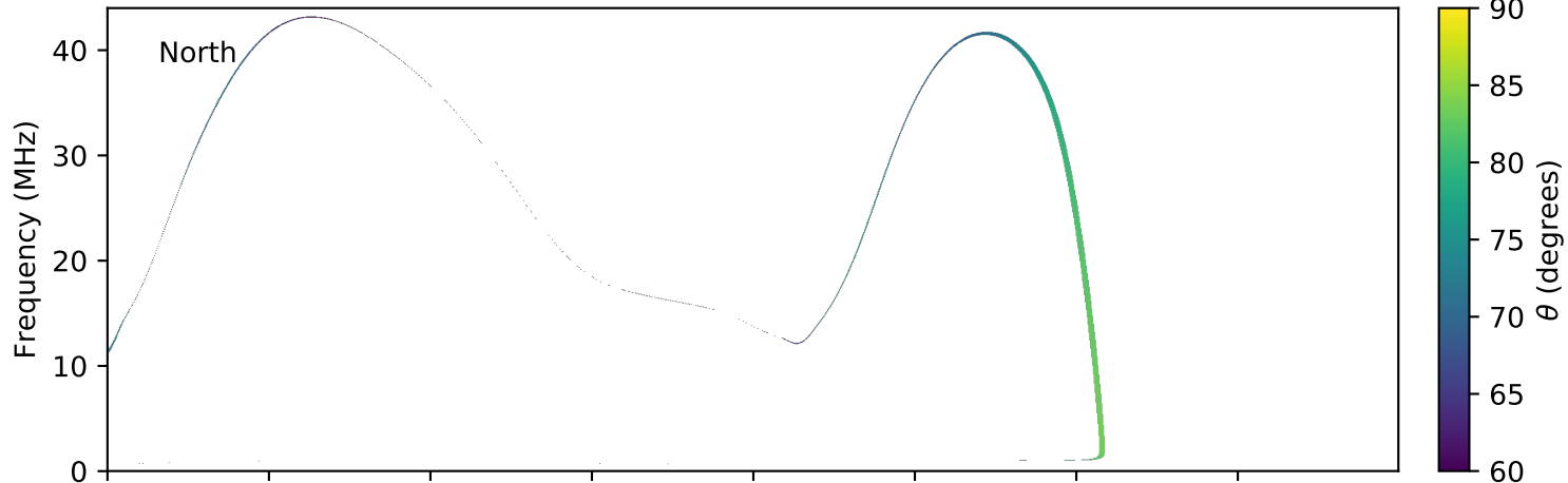
expres_earth_jupiter_io_jrm09_lossc-wid1deg_3kev_20100822_v01.cdf
